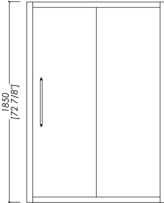
MAS/130 (128-132) | (50 3/8"-52")
