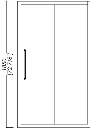
MAS/110 (108-112) | (42 1/2"-44 1/8")
