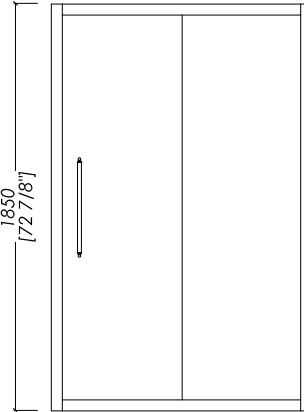
MAS/120 (118-122) | (46 1/2"-48")
